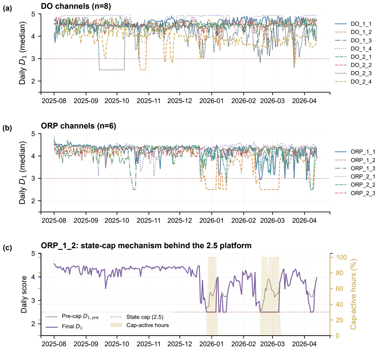
Figure 7. Daily sensor-health trajectories and state-cap interpretation
